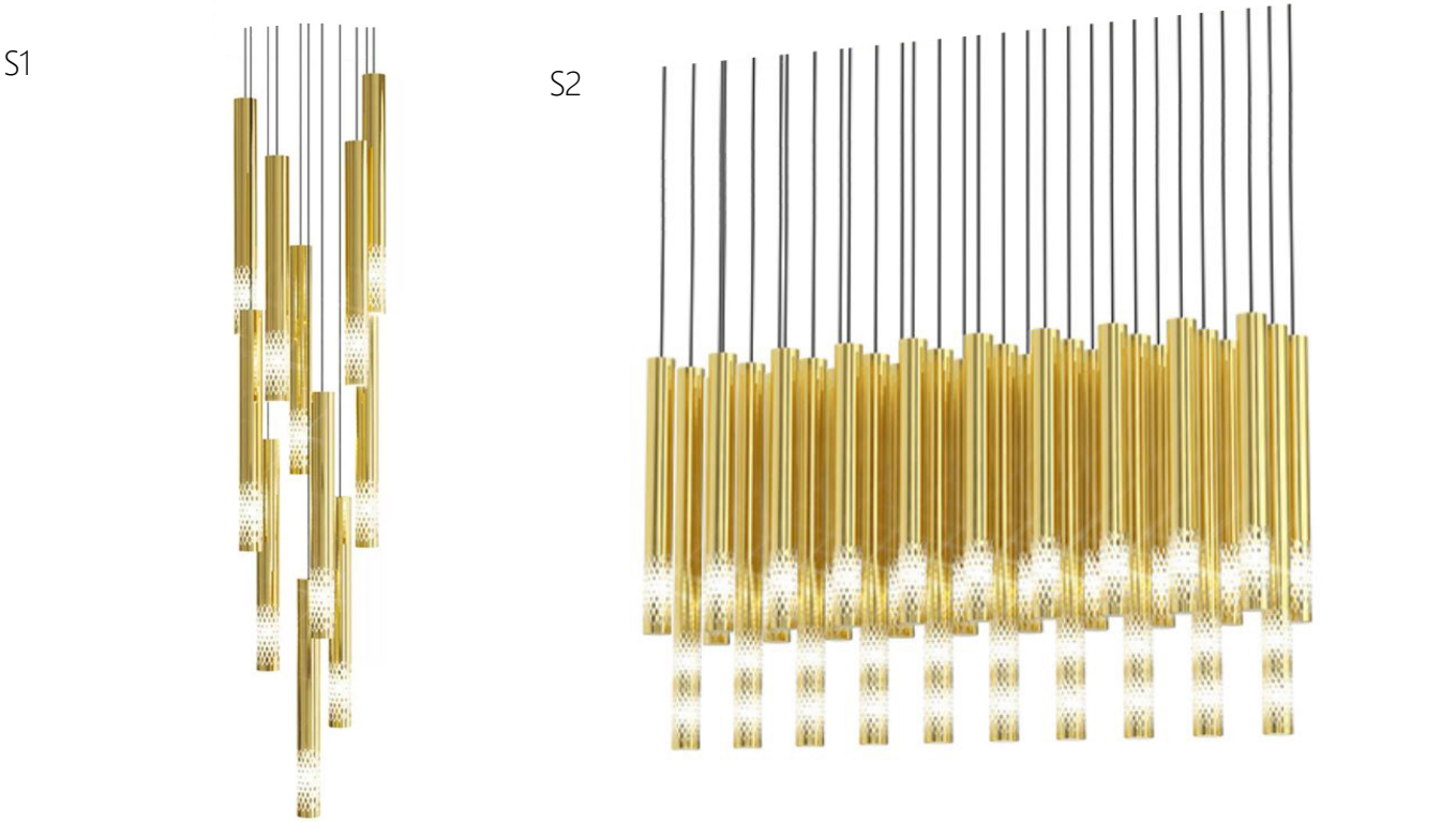
Spirit S 1 Spirit S 2 Size : Dia 300 x H 1250 x OH 1400 mm Size : L 1100 x W 400 x H 600 x OH 1000 mm Colours : Crystal aurum Colours : Crystal aurum Light sources : 11 pcs G9 Light sources : 30 pcs G9
